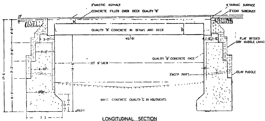
Fig. 339.—Longitudinal Section.
